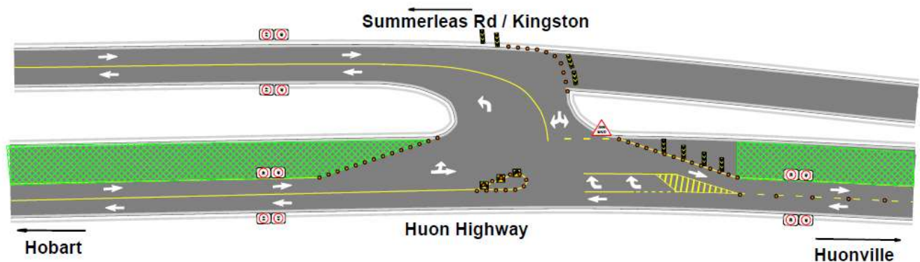
Figure 2: New Summerleas Road/Kingston Intersection
