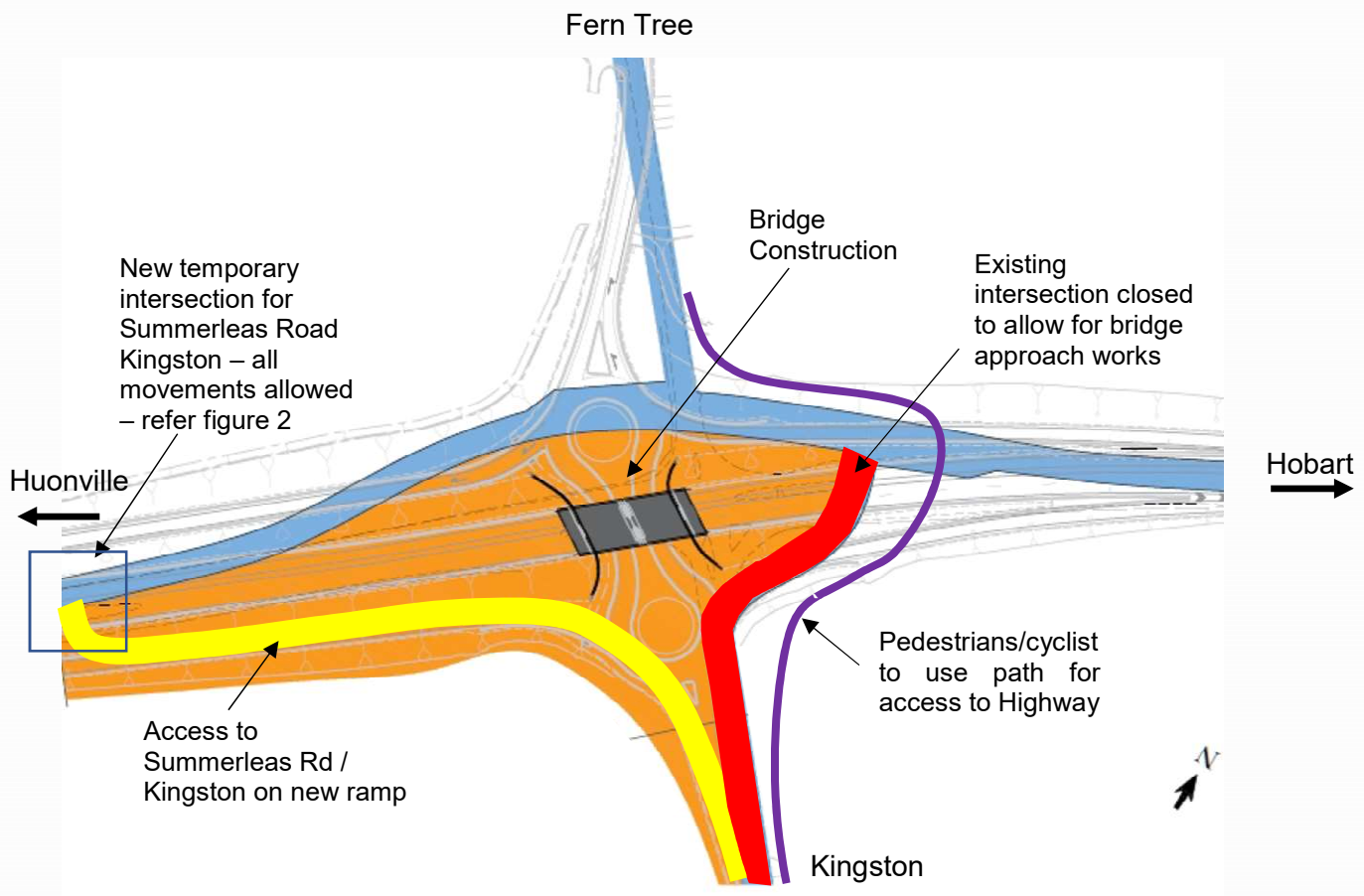
Figure 1: Moved Summerleas Road/Kingston Intersection
