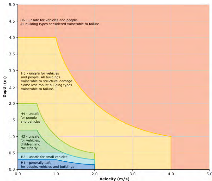
Figure 30: Combined Flood Hazard Curves (Ball et al., 2016)
