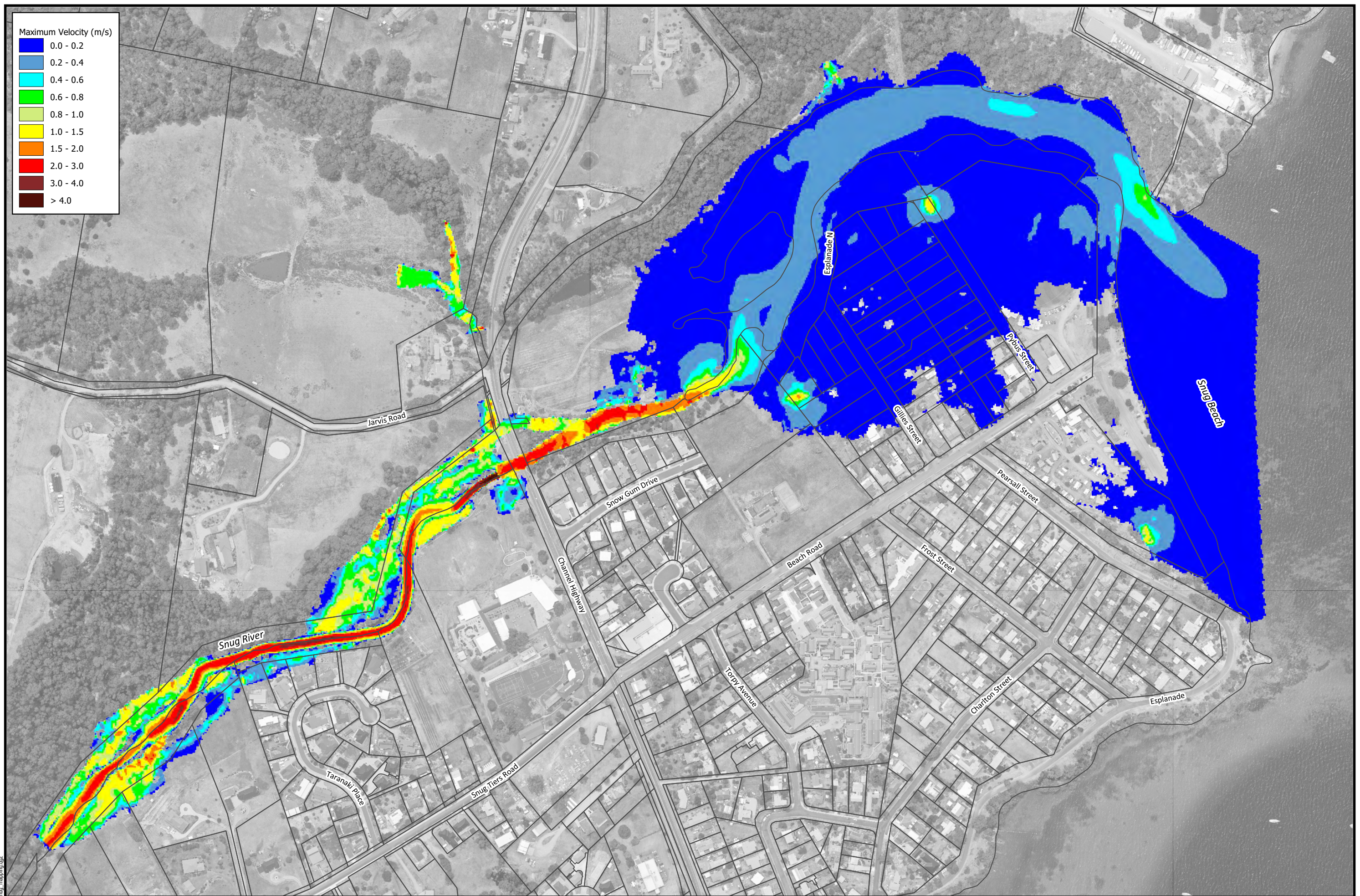
Figure B-11 Peak Velocities | 2050 Climate Change Analysis 5% AEP Catchment Event +10% Rainfall Increase with 1% AEP Tailwater +0.30m SLR
