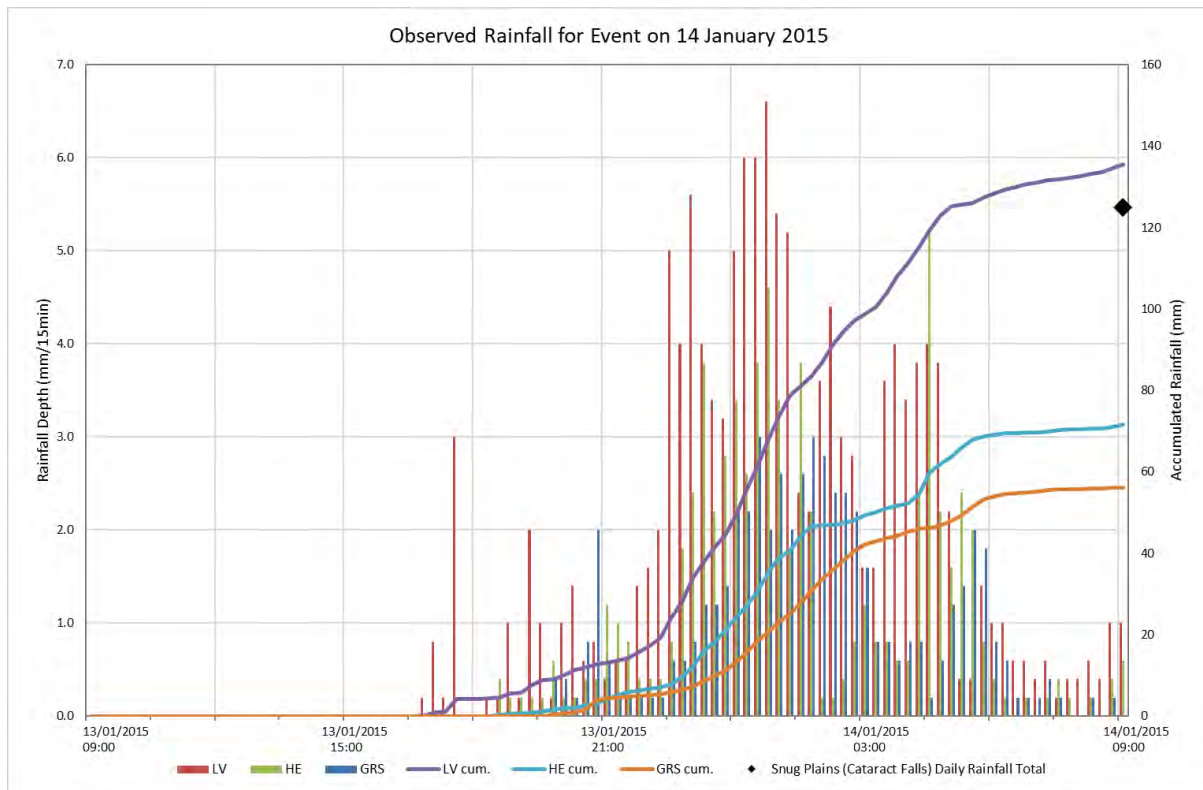
Figure 22: Recorded Rainfall – January 2015 Event
