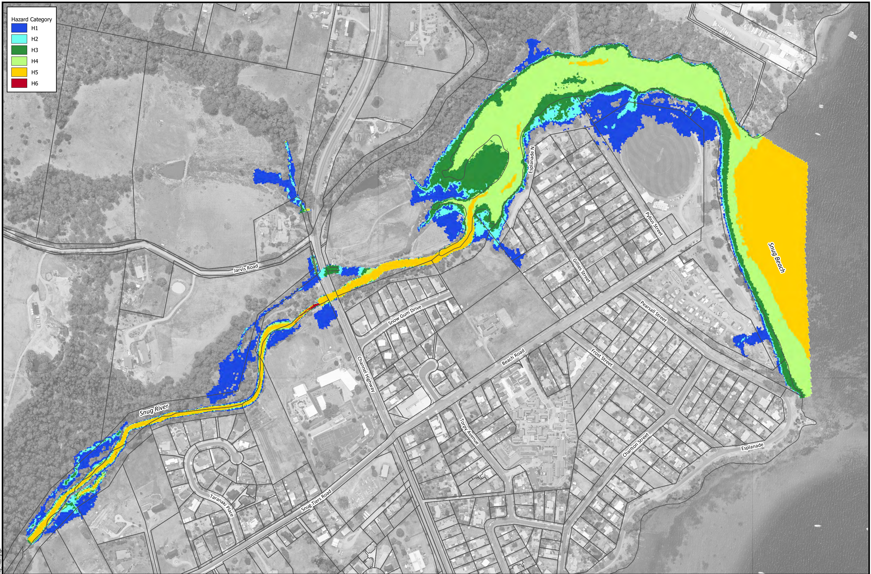
Figure A-16 Peak Hazard Category | 20% AEP Catchment Event + 20% AEP Tailwater
