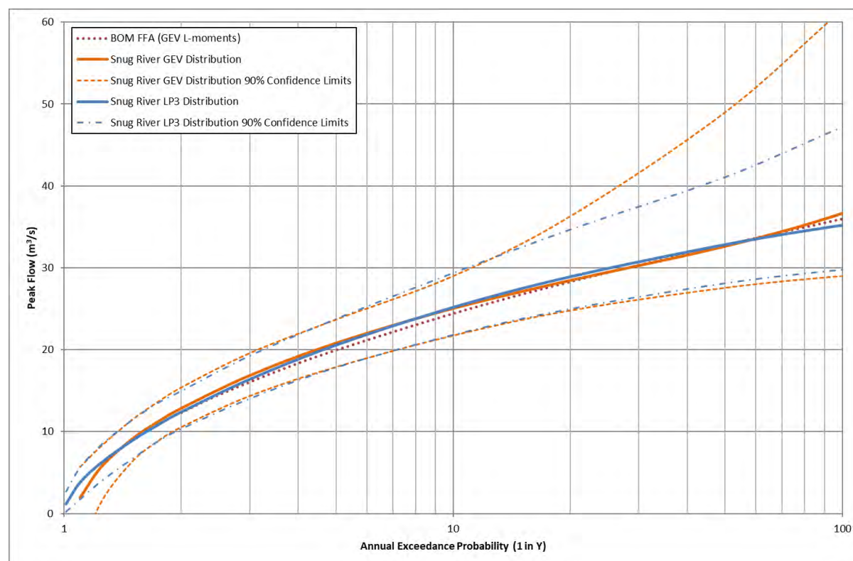
Figure 28: Snug River Flood Frequency Curves
