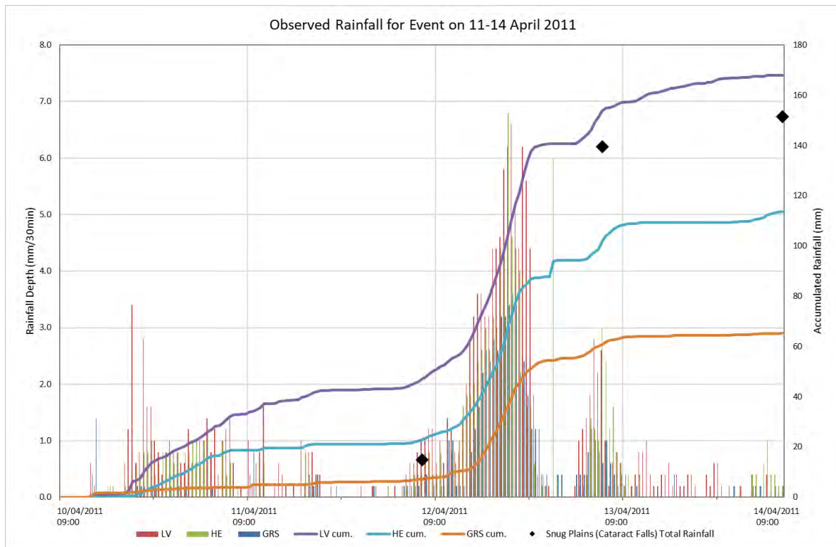
Figure 18: Recorded Rainfall – April 2011 Event
