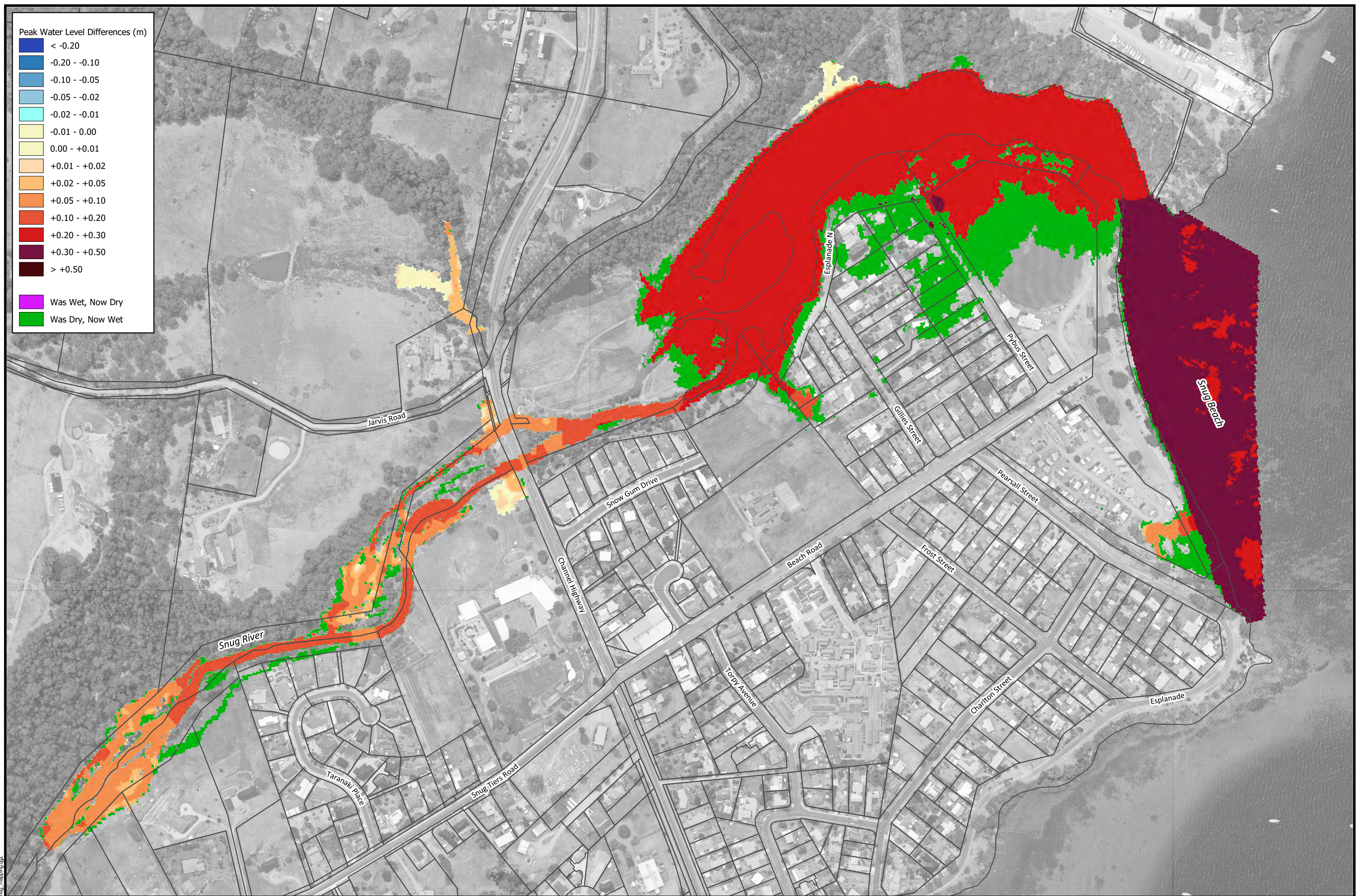
Figure B-20 Peak Water Level Differences | 2050 Climate Change Analysis 20% AEP Catchment Event +10% Rainfall Increase with 20% AEP Tailwater +0.30m SLR
