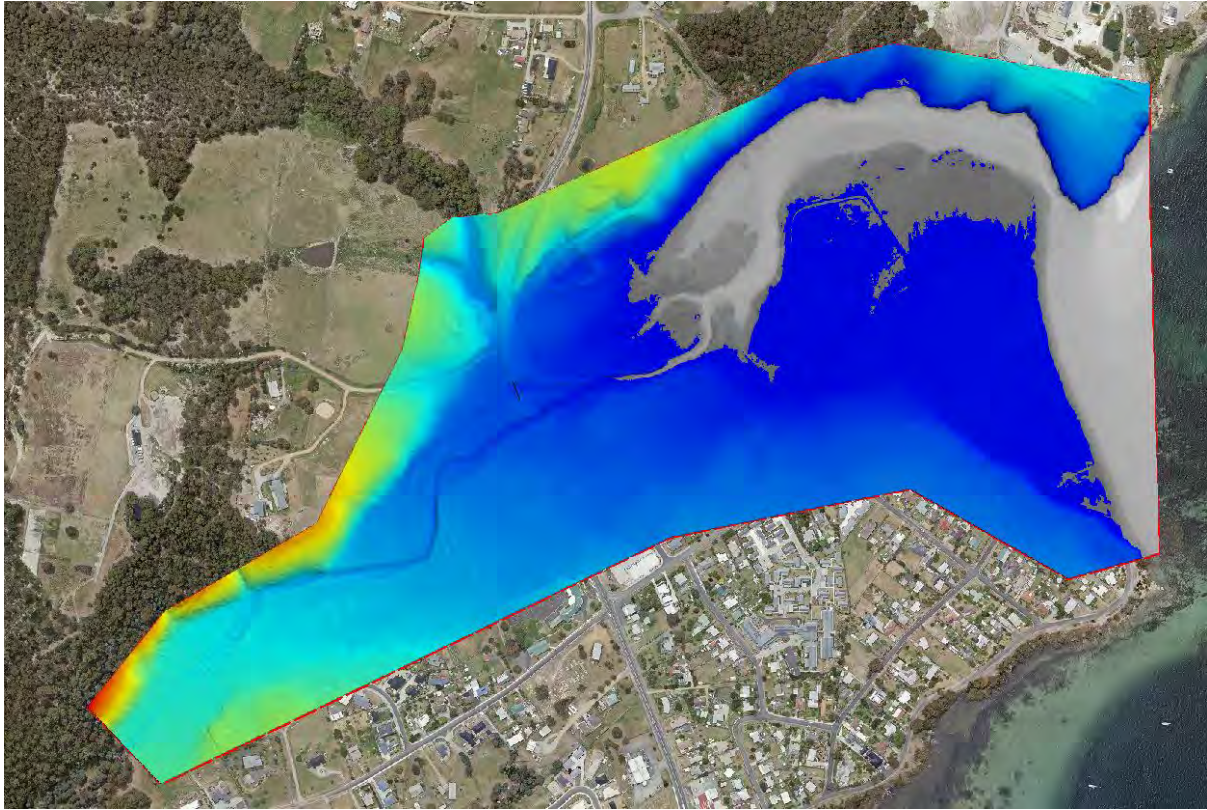
Figure 14: Hydraulic Model Topography
