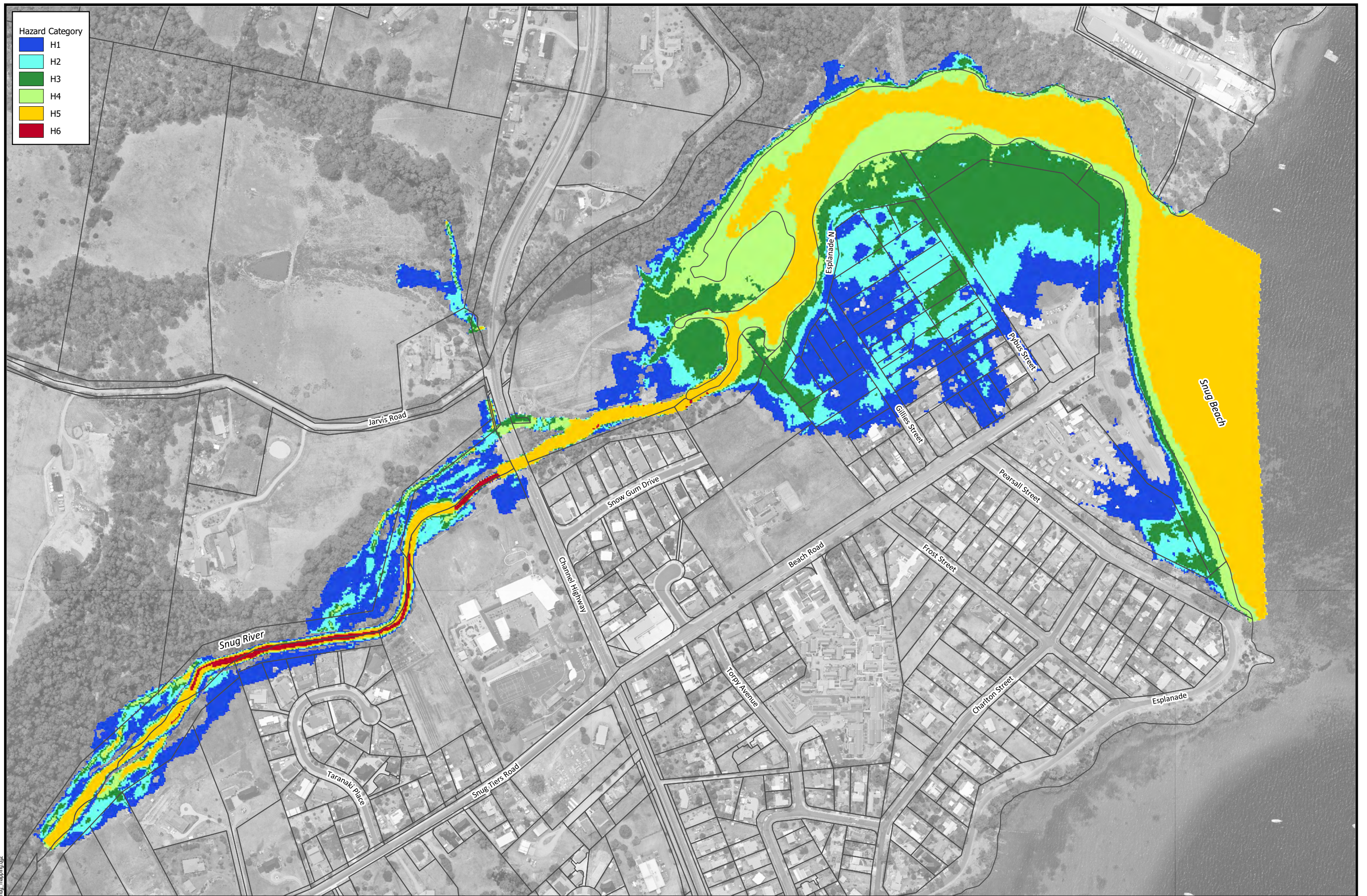
Figure B-15 Peak Hazard Category | 2050 Climate Change Analysis 5% AEP Catchment Event +10% Rainfall Increase with 1% AEP Tailwater +0.30m SLR
