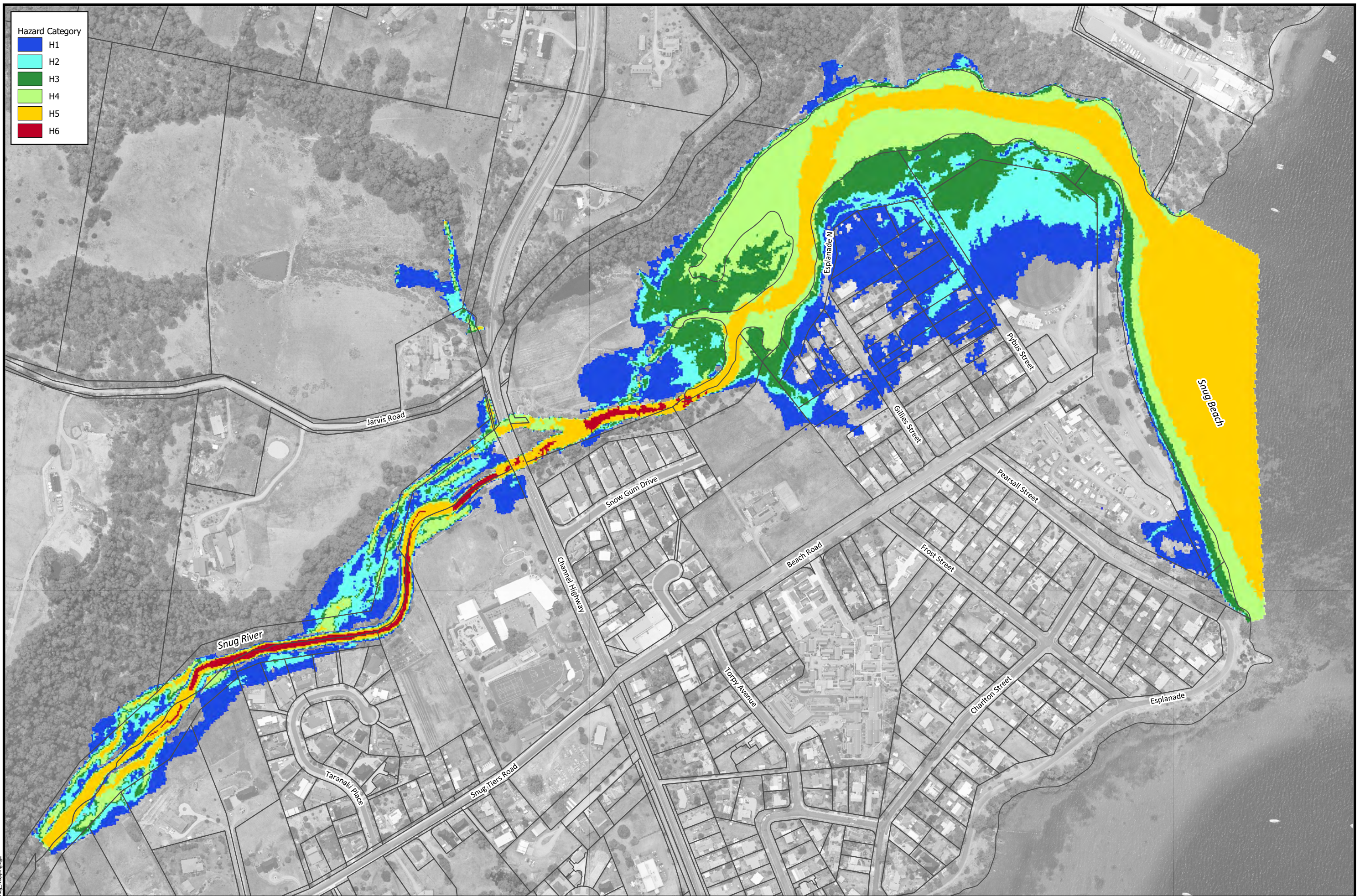
Figure A-14 Peak Hazard Category | 1% AEP Catchment Event + 5% AEP Tailwater
