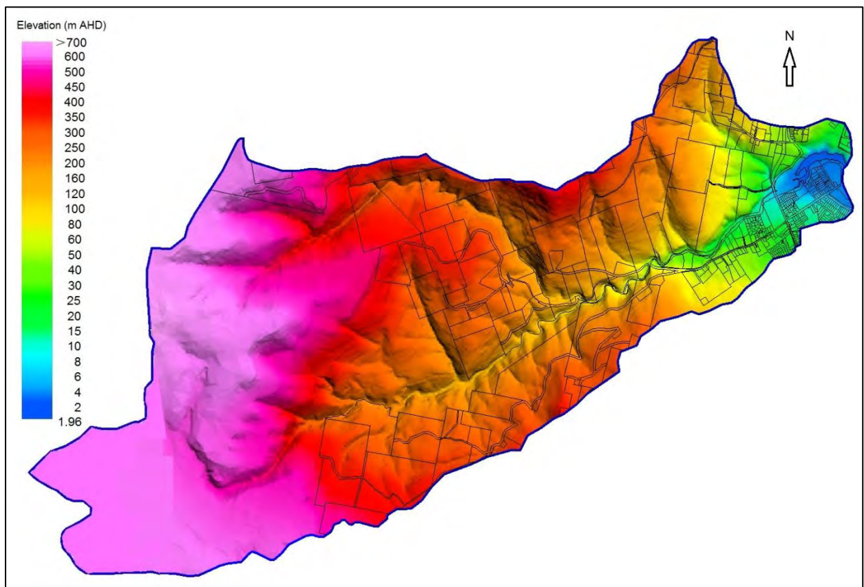
Figure 8: The elevation of Snug Catchment.
