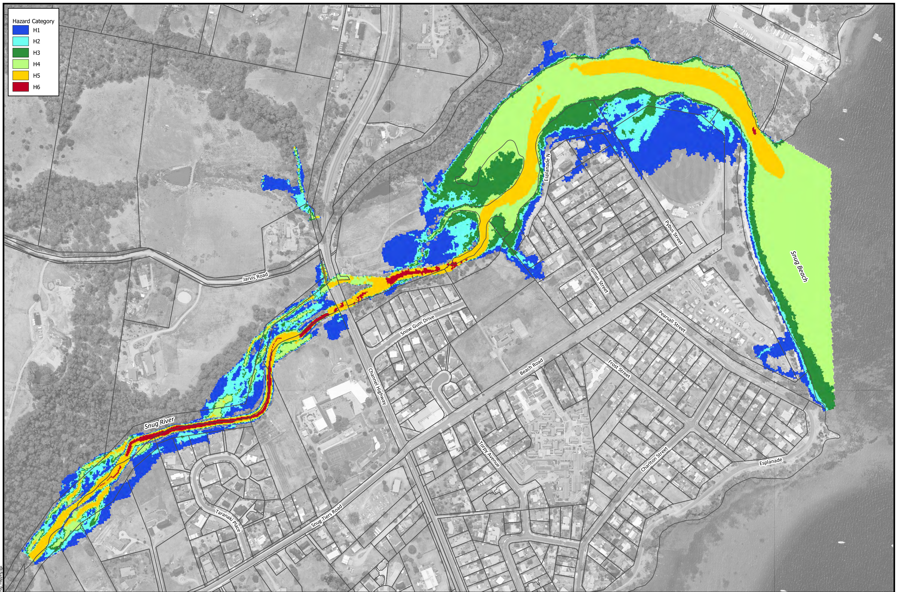
Figure A-13 Peak Hazard Category | 1% AEP Catchment Event + MHWS Tailwater
