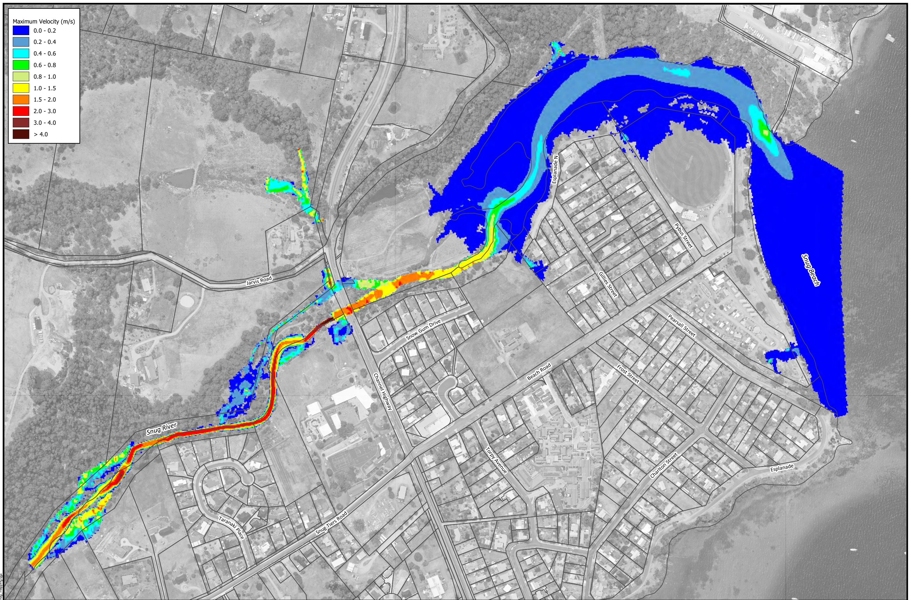
Figure A-12 Peak Velocities | 20% AEP Catchment Event + 20% AEP Tailwater
