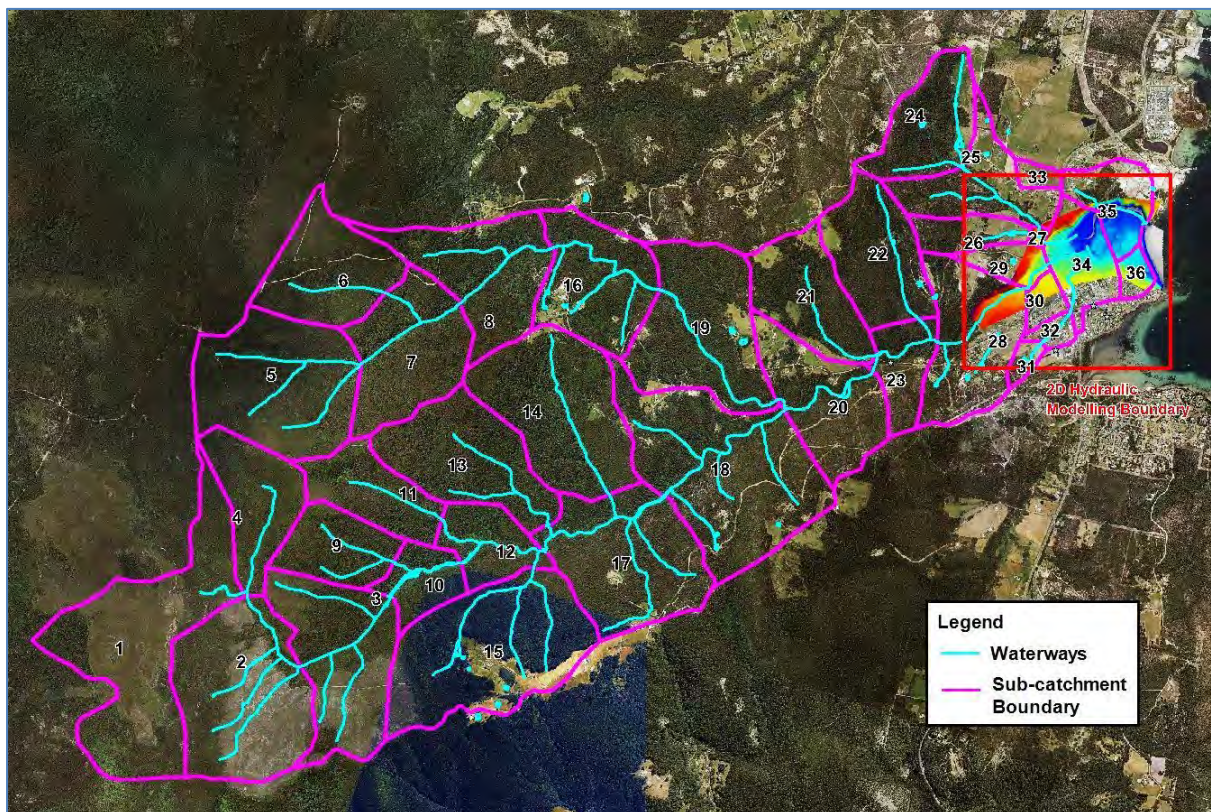
Figure 12: Hydrologic and Hydraulic Model Extents
