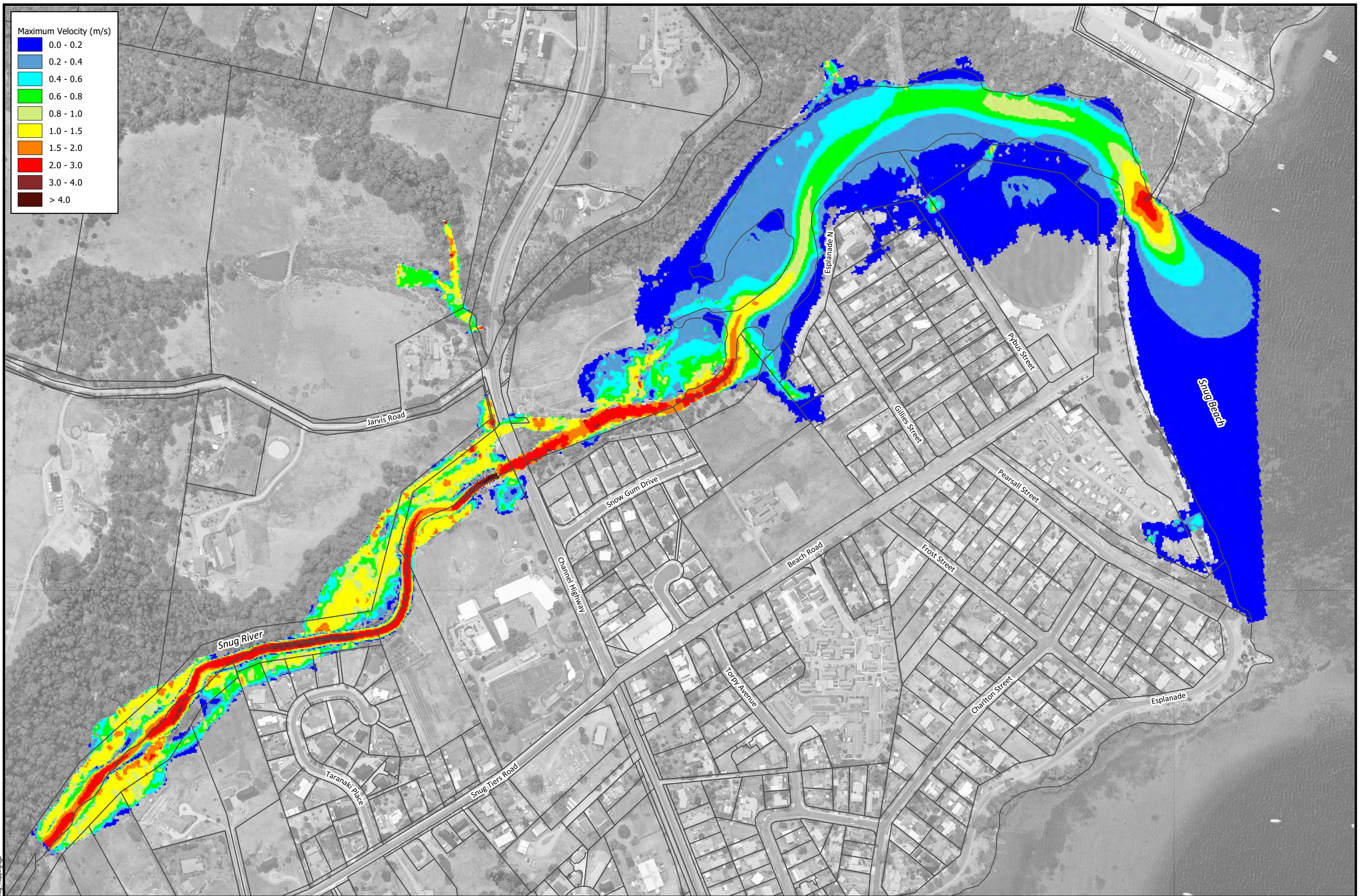
Figure A-09 Peak Velocities | 1% AEP Catchment Event + MHS Tailwater
