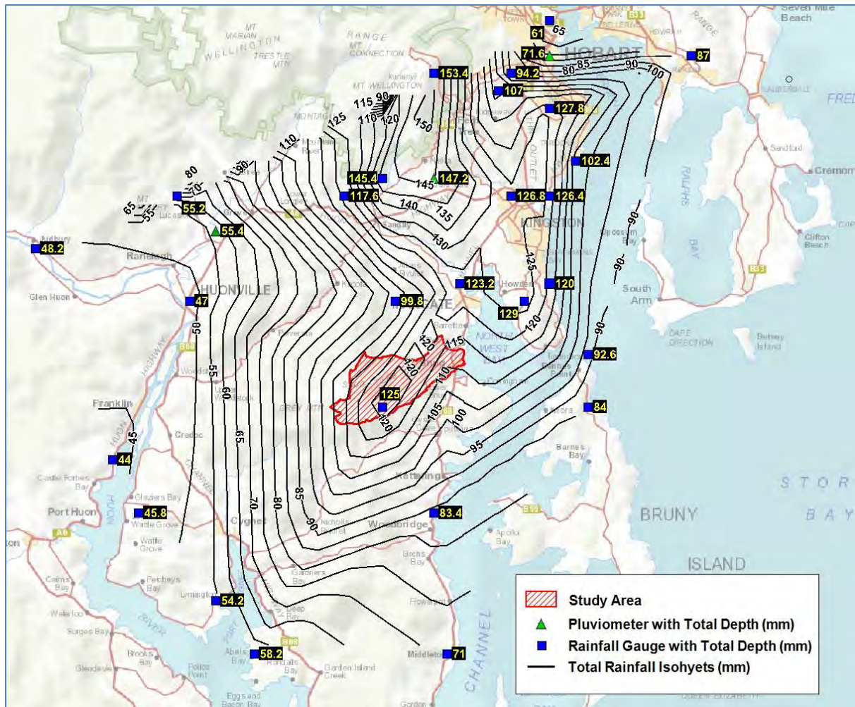
Figure 21: Rainfall Distribution for 14 January 2015
