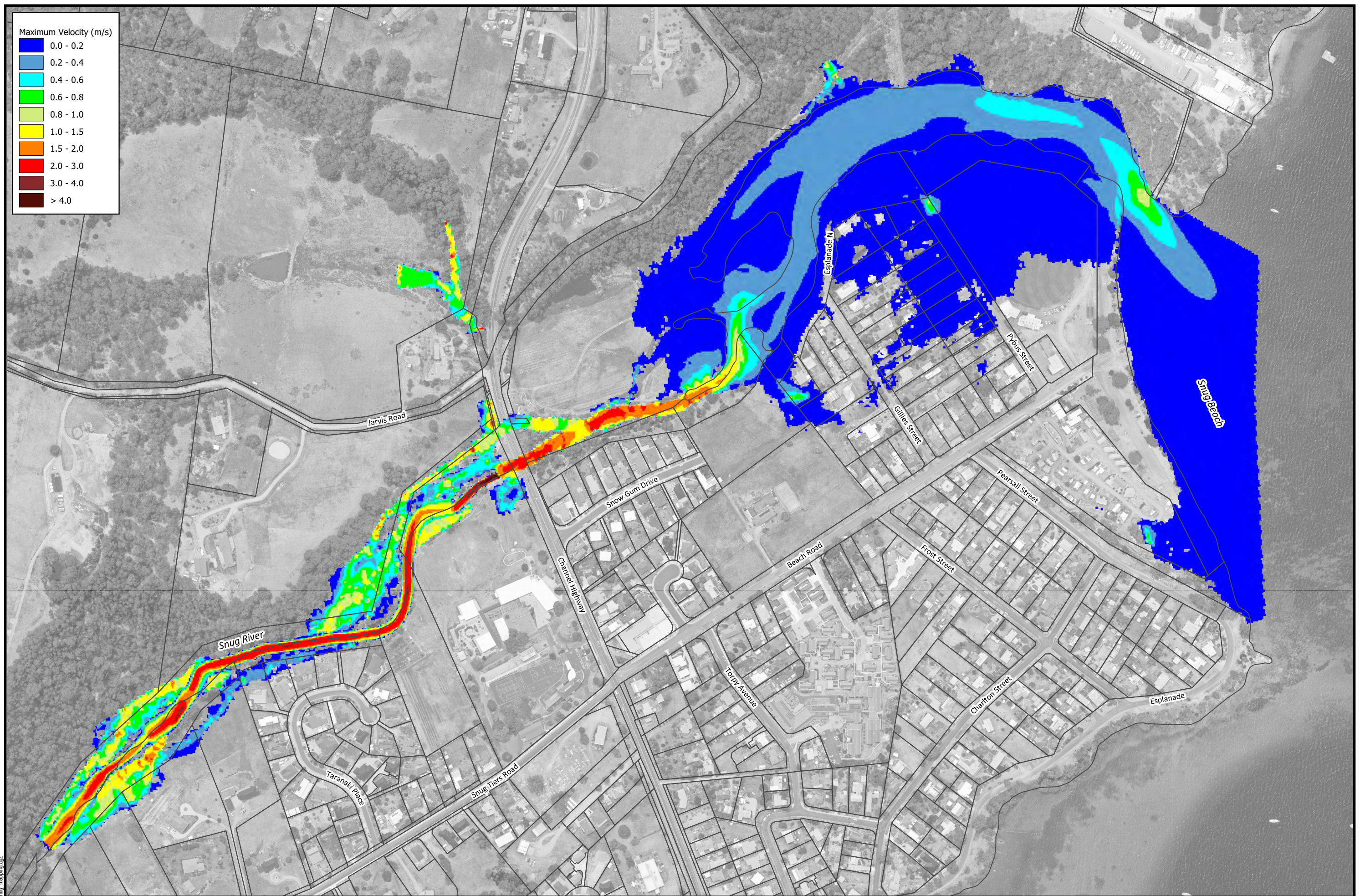
Figure A-11 Peak Velocities | 5% AEP Catchment Event + 1% AEP Tailwater
