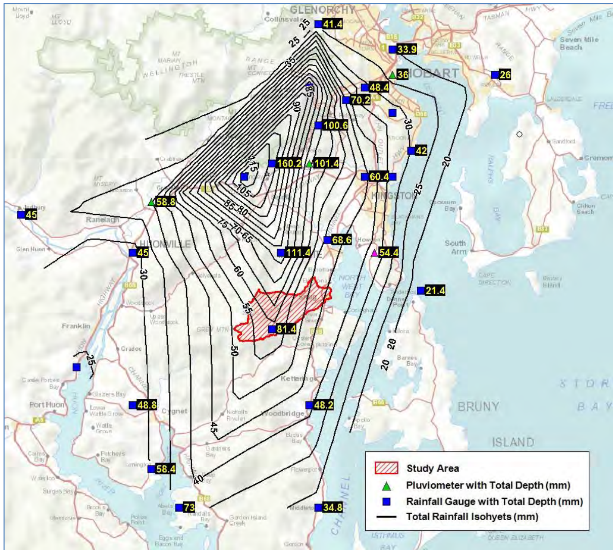
Figure 25: Rainfall Distribution for 7 June 2016
