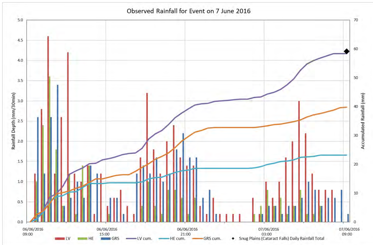
Figure 26: Recorded Rainfall – June 2016 Event
