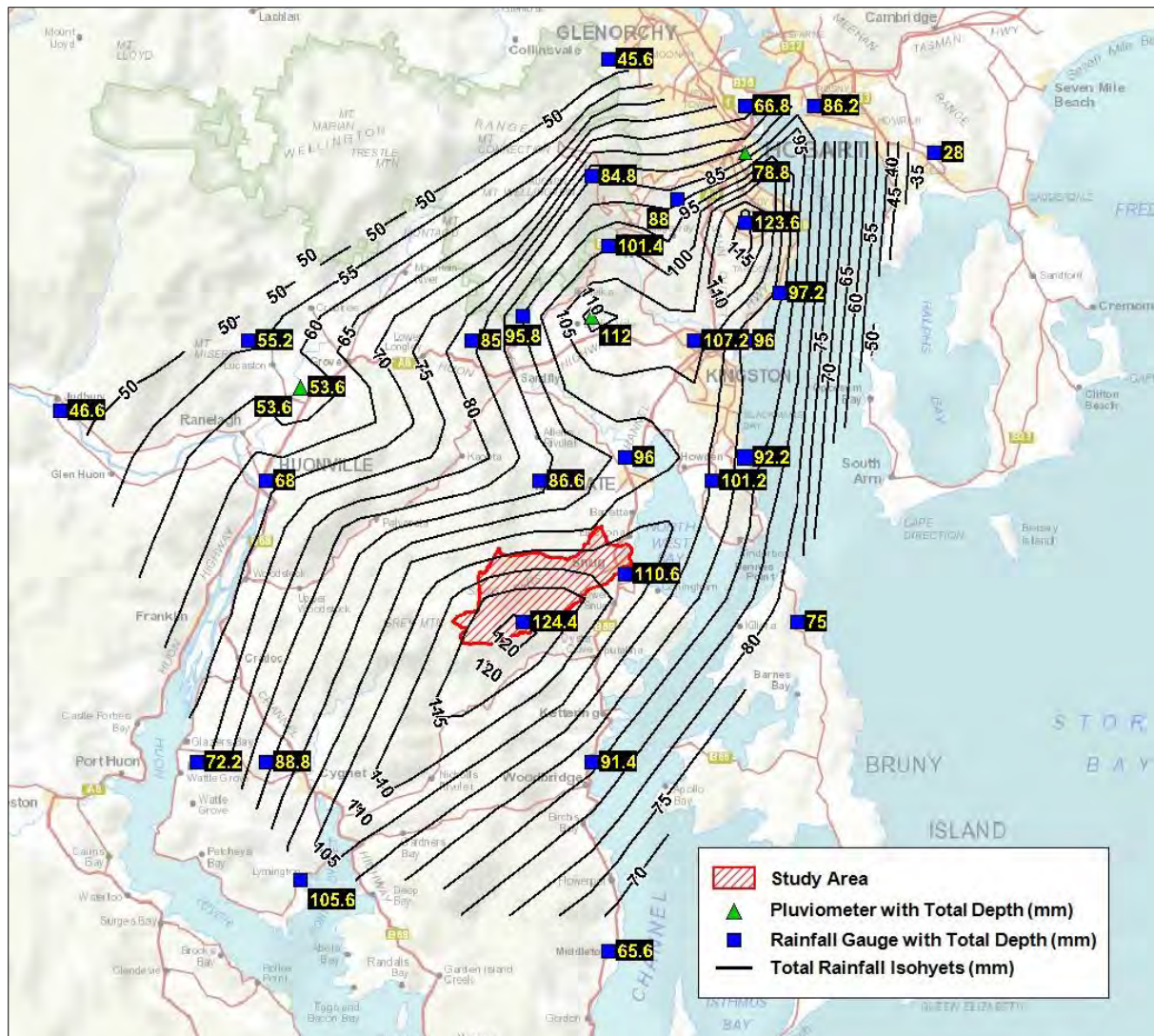
Figure 17: Rainfall Distribution for 13 April 2011
