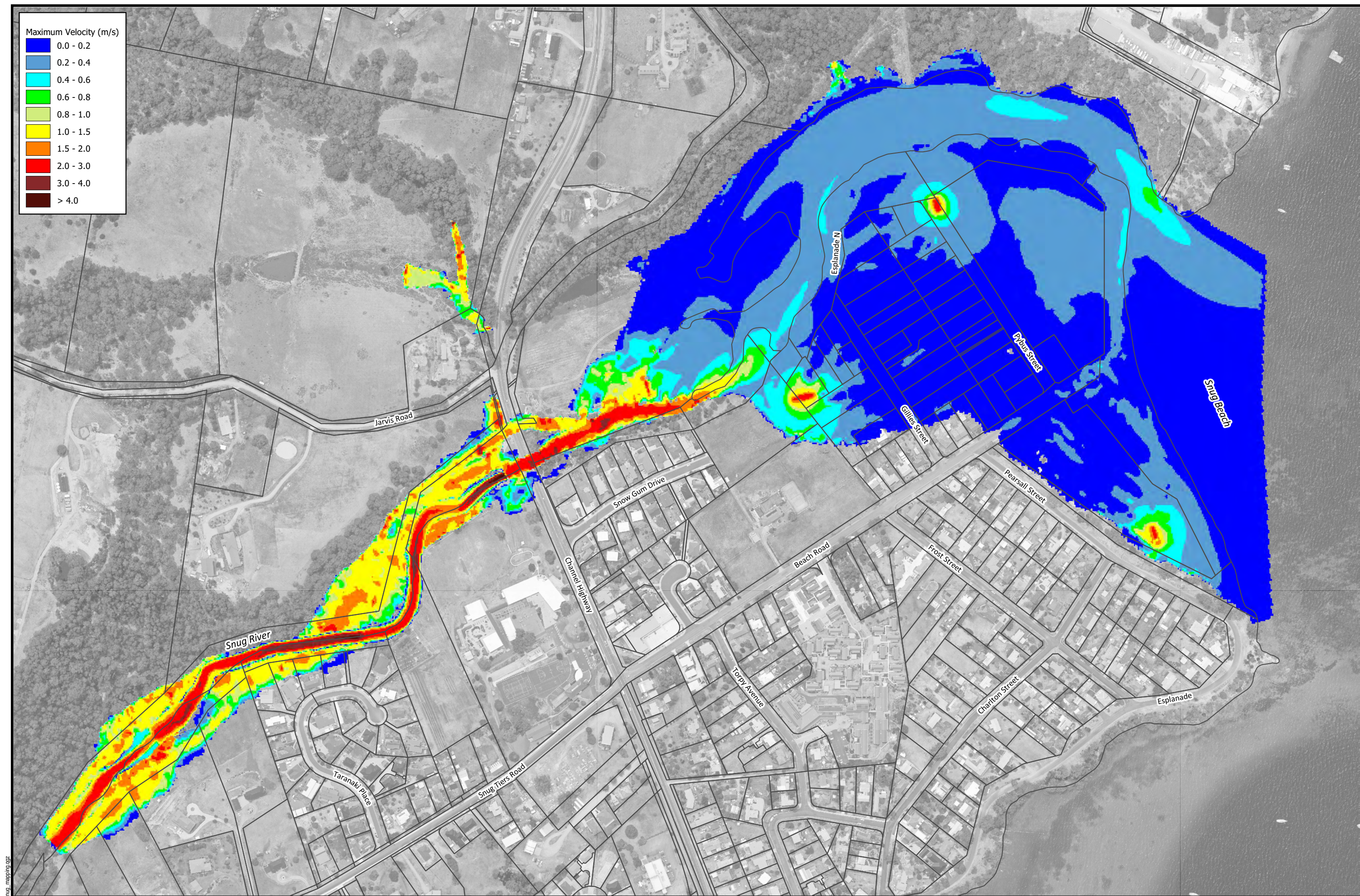
Figure C-10 Peak Velocities | 2100 Climate Change Analysis 1% AEP Catchment Event +30% Rainfall Increase with 5% AEP Tailwater +1.00m SLR
