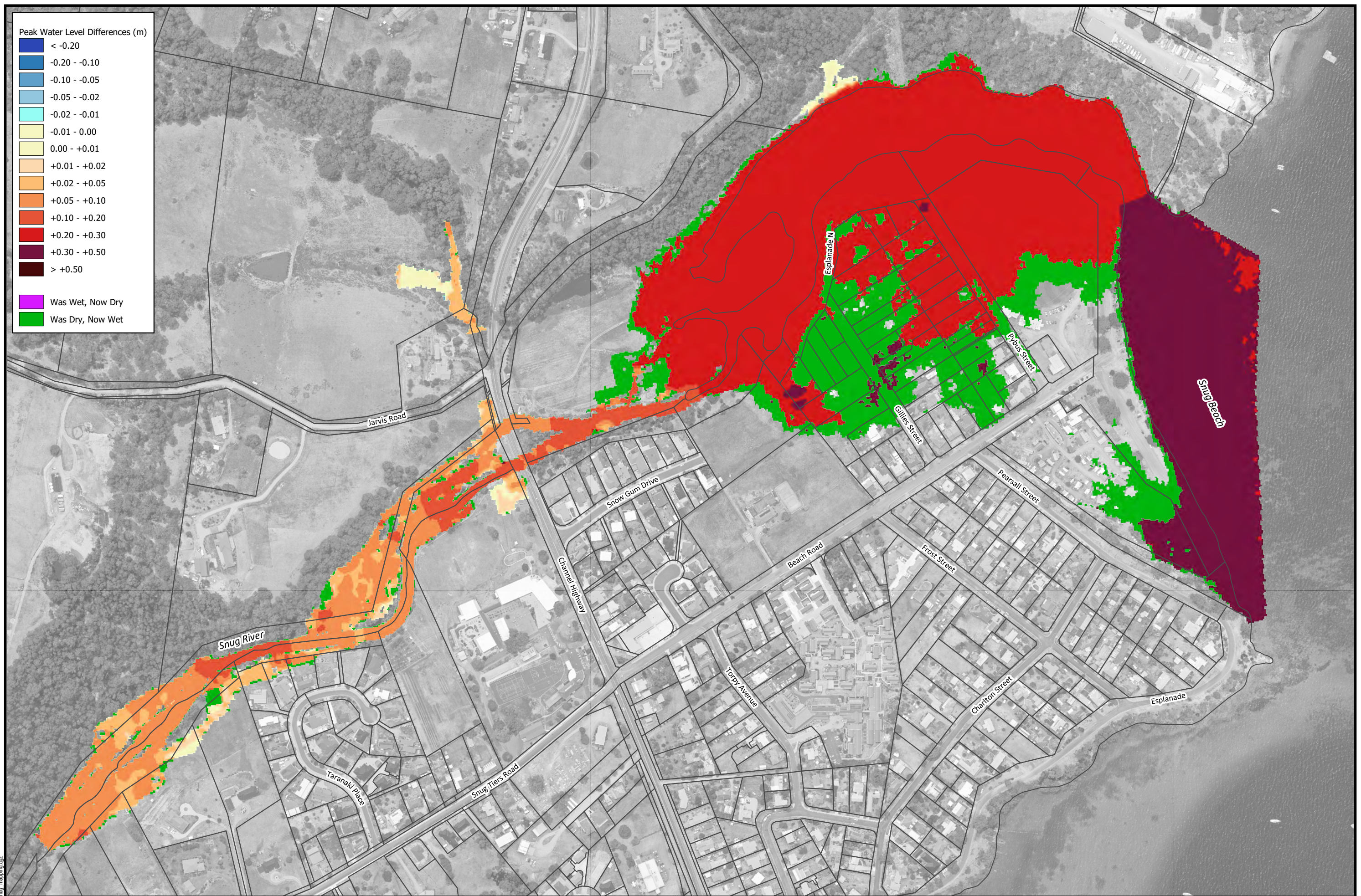
Figure B-19 Peak Water Level Differences | 2050 Climate Change Analysis 5% AEP Catchment Event +10% Rainfall Increase with 1% AEP Tailwater +0.30m SLR
