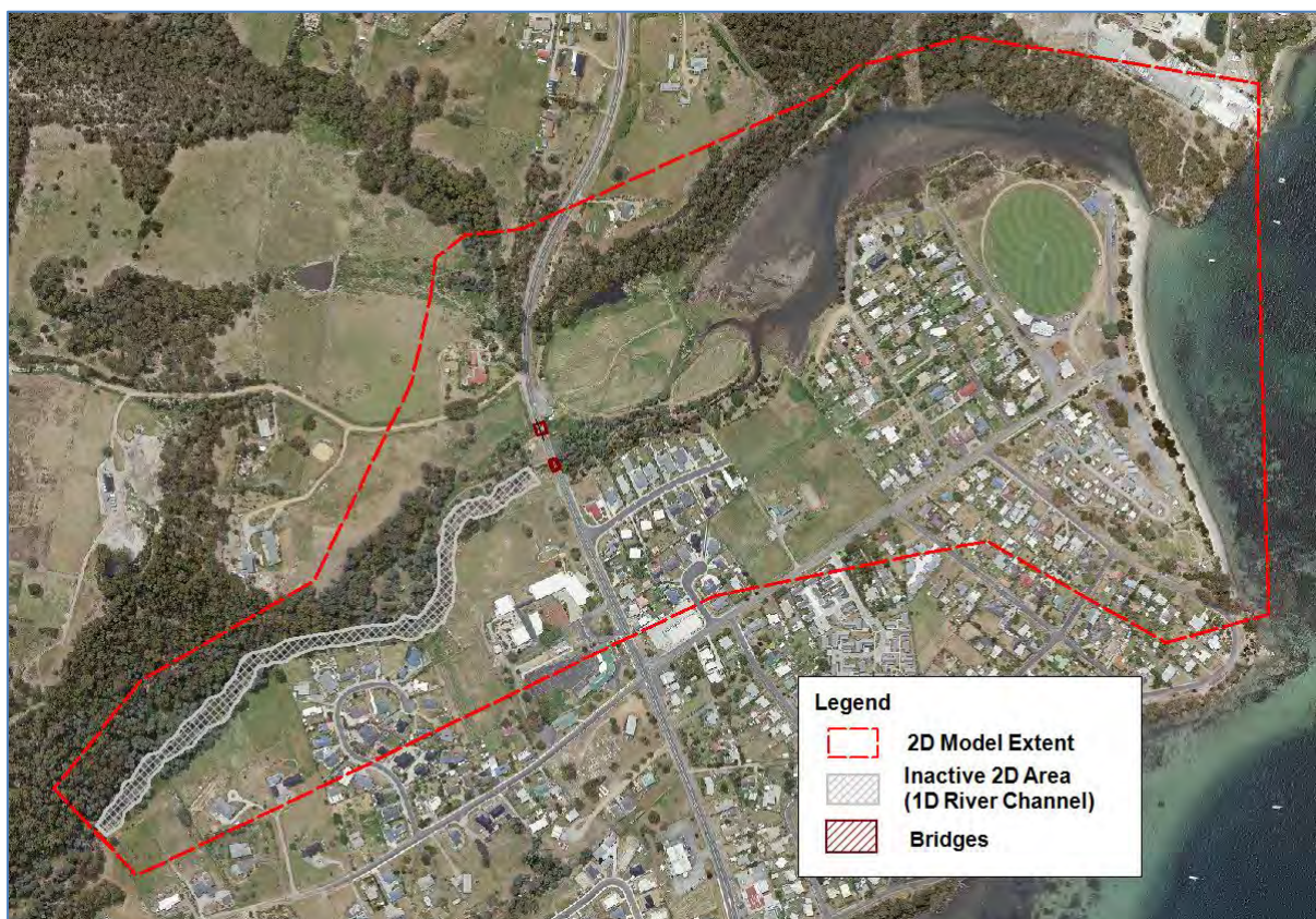
Figure 13: Hydraulic Model Extents
