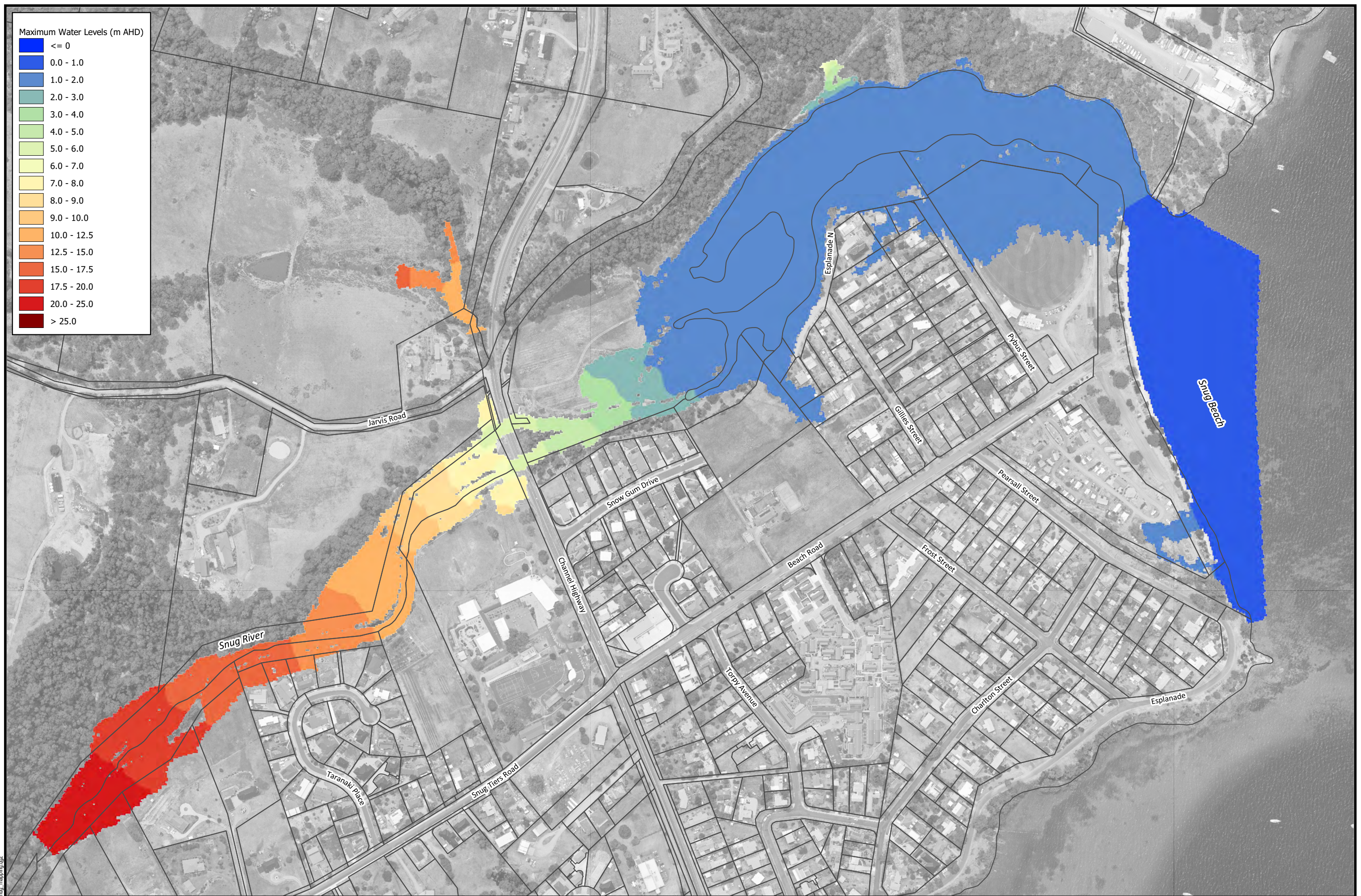
Figure A-01 Peak Water Levels | 1% AEP Catchment Event + MHWs Tailwater
