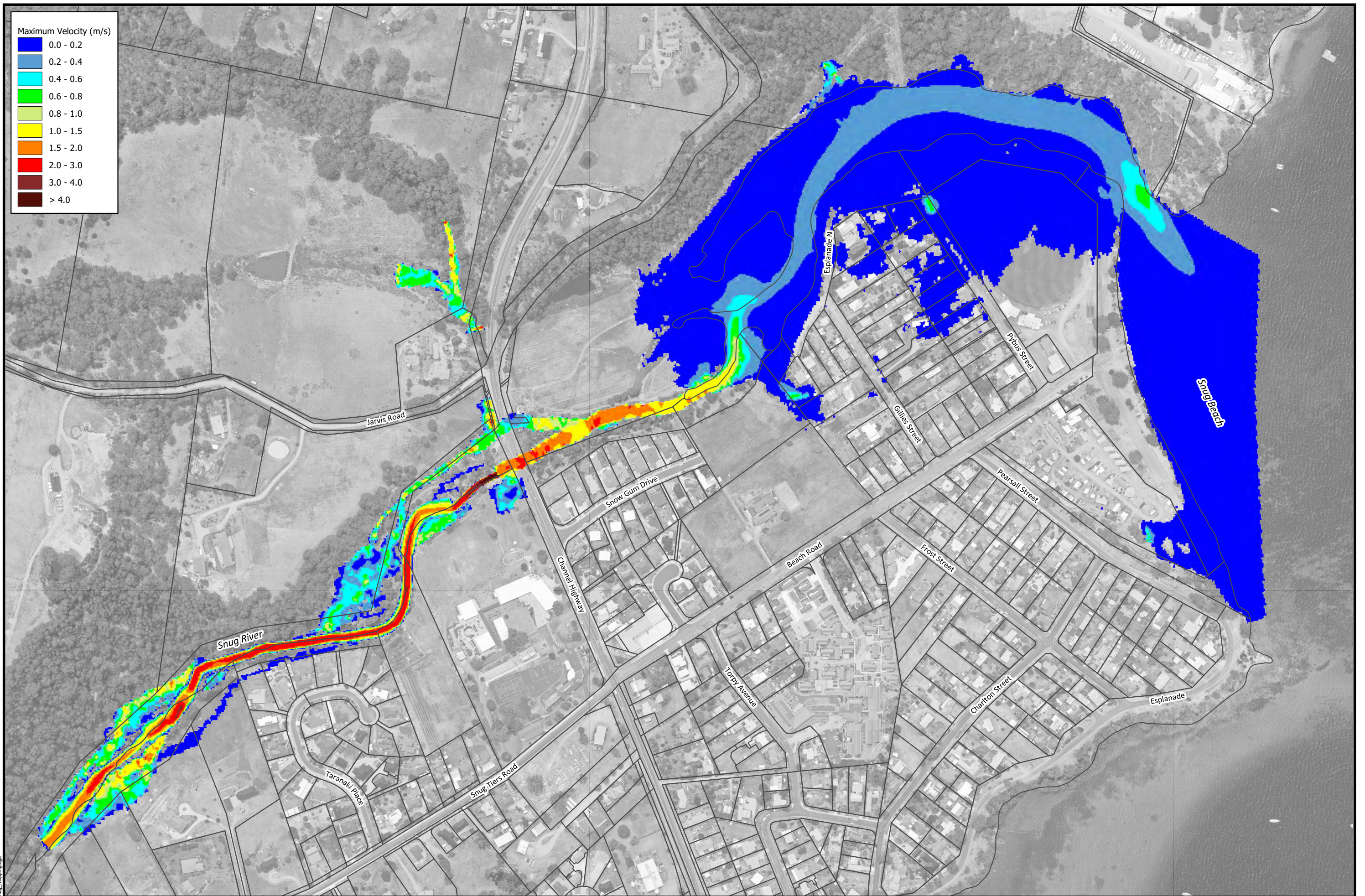
Figure B-12 Peak Velocities | 2050 Climate Change Analysis 20% AEP Catchment Event +10% Rainfall Increase with 20% AEP Tailwater +0.30m SLR
