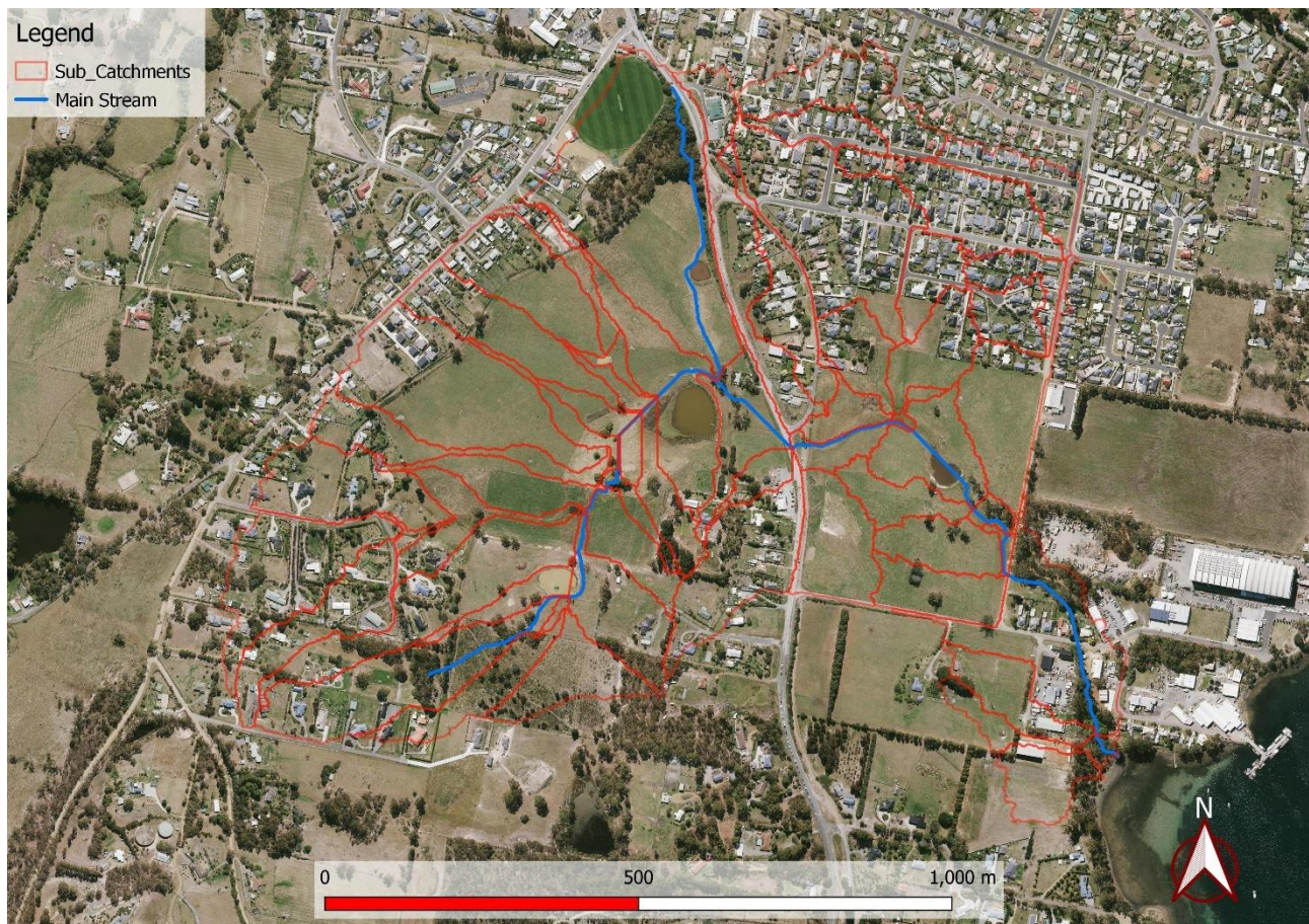
Figure 4. Tramway Creek Hydrology sub-catchments
